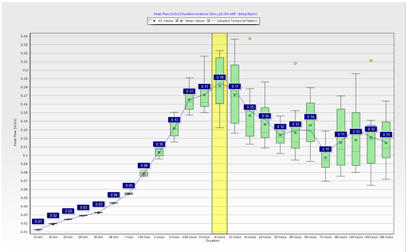
Figure 39. Treatment Inflows
